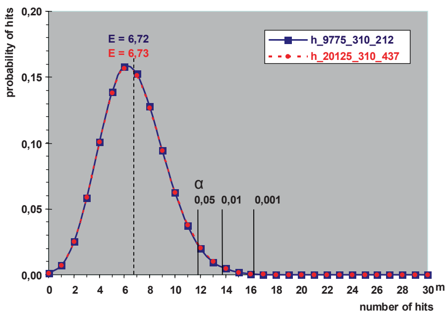
Fig. 1. Hypergeometric distribution: probability to have hits in a battleship with 310 ships on a grid of N = 9,775 (or 20,125, respectively) fields with 212 (or 437, respectively) shots; \alpha represents the chance to be outside of the area under the curve (e.g. chance of 17 hits or more is below \alpha = 0.001 ) [10].
