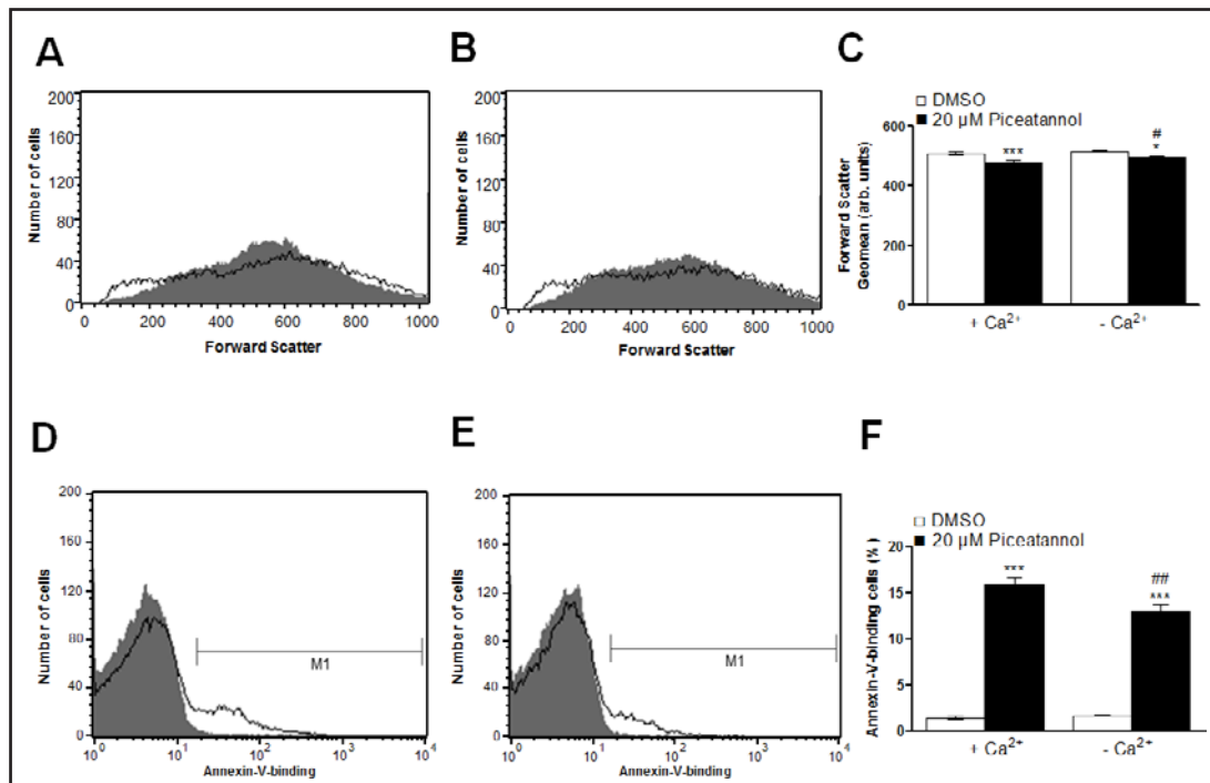
Fig. 3. Ca^{2+} sensitivity of Piceatannol-induced erythrocyte shrinkage and phosphatidylserine exposure. A,B. Original histogram of forward scatter of erythrocytes following exposure for 48 hours to Ringer solution without (grey area) and with (black line) Piceatannol (20 \mu M) in the presence (A) and absence (B) of extracellular Ca^{2+} . C. Arithmetic means \pm SEM (n = 10) of forward scatter of erythrocytes after a 48 hours treatment with Ringer solution without (white bars) or with (black bars) Piceatannol (20 \mu M) in the presence (left bars, +Ca^{2+} ) and absence (right bars, -Ca^{2+} ) of Ca^{2+} . D,E. Original histogram of annexin-V-binding of erythrocytes following exposure for 48 hours to Ringer solution without (grey area) and with (black line) Piceatannol (20 \mu M) in the presence (D) and absence (F) of extracellular Ca^{2+} . F. Arithmetic means \pm SEM (n = 10) of annexin-V-binding of erythrocytes after a 48 hours treatment with Ringer solution without (white bars) or with (black bars) Piceatannol (20 \mu M) in the presence (left bars, +Ca^{2+} ) and absence (right bars, -Ca^{2+} ) of Ca^{2+} . *(p<0.05), *** (p<0.001) indicates significant difference from the absence of Piceatannol, # (p<0.05), ## (p<0.01) indicates significant difference from the nominal absence of Ca^{2+} (ANOVA).
